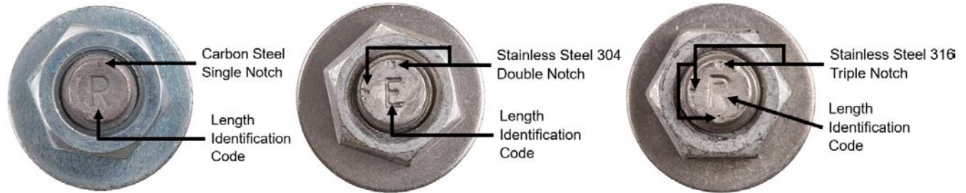
FIGURE 4—BOLT HEAD WITH LENGTH IDENTIFICATION CODE AND KB-TZ2 HEAD NOTCH EMBOSMENT
